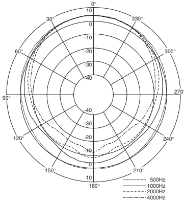
Polar Response (Horizontal)
